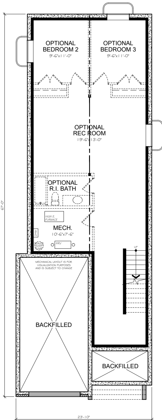
BASEMENT PLAN
